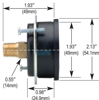
20-110 Panel Mount Clamp
