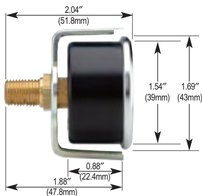
15-110 Panel Mount Clamp
