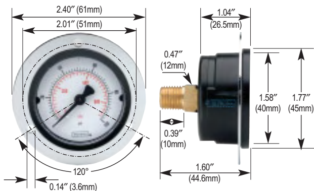
15-110 Front Flange
