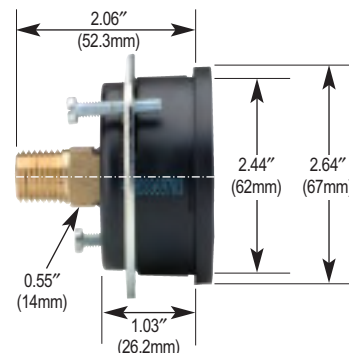
25-110 Panel Mount Clamp
