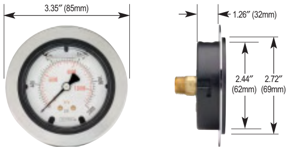
25-910 Panel Mount Clamp
