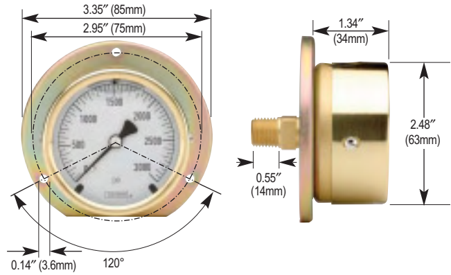
25-310 Rear Flange
