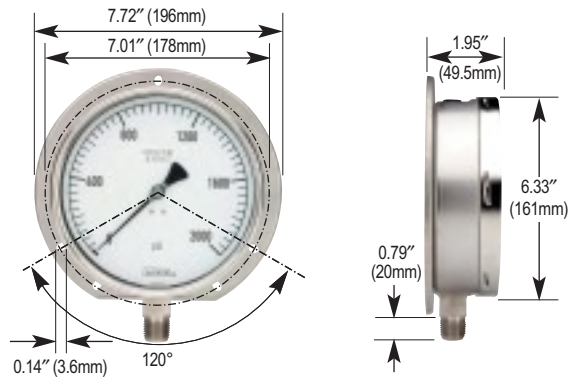
60-410/510 Rear Flange
