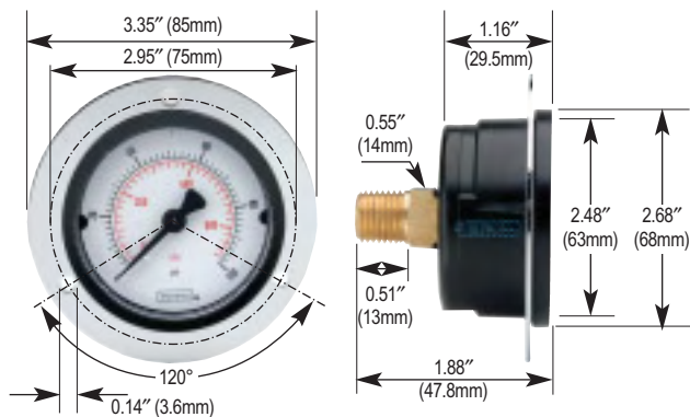
25-110 Front Flange
