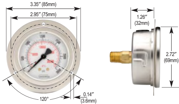
25-910 Flange Ring
