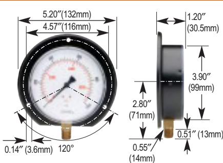
40-100 Rear Flange
