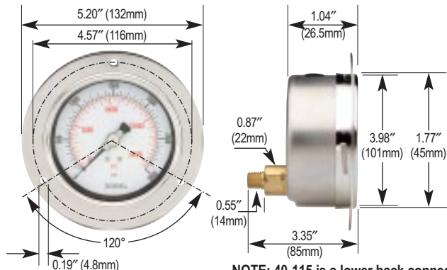
40-115 Front Flange
