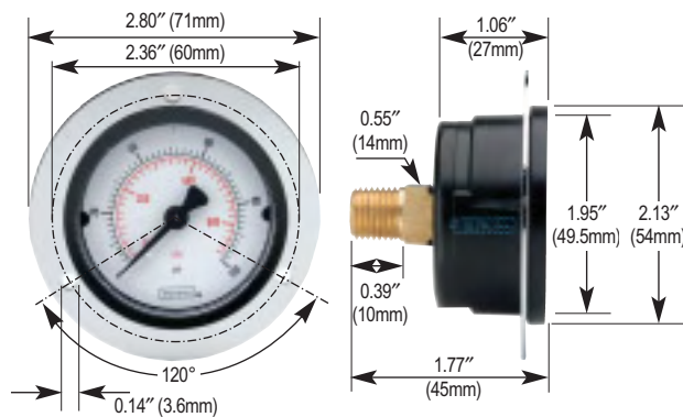
20-110 Front Flange
