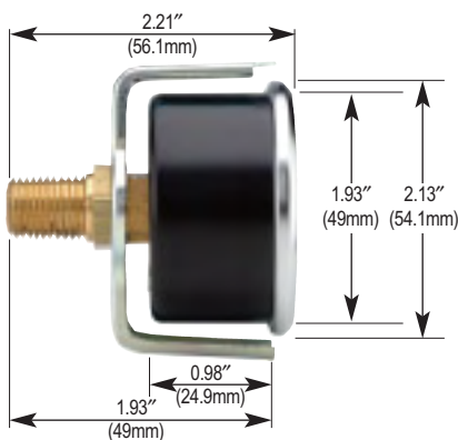
20-110 Panel Mount Clamp
