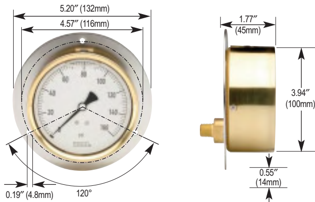
40-310 Rear Flange
