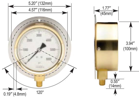
40-300 Rear Flange
